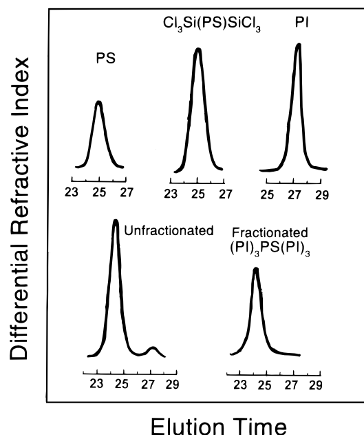
Figure 1. SEC chromatograms of the SH10-20 block copolymer.
